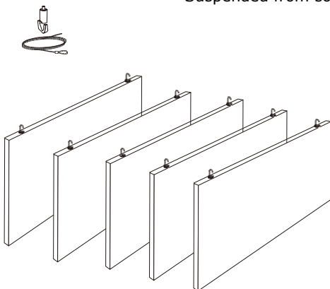
Installation Method 1: ISpring Anchor Fixture Kit Suspended from soffit
