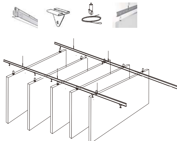
Method 2 : Suspended from T sub-frame
